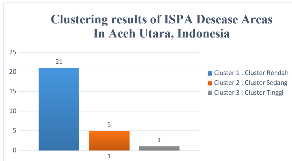
Figure 2. Cluster Graph
